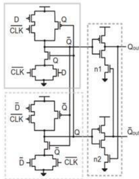
Fig 2: Proposed MRF Latch
