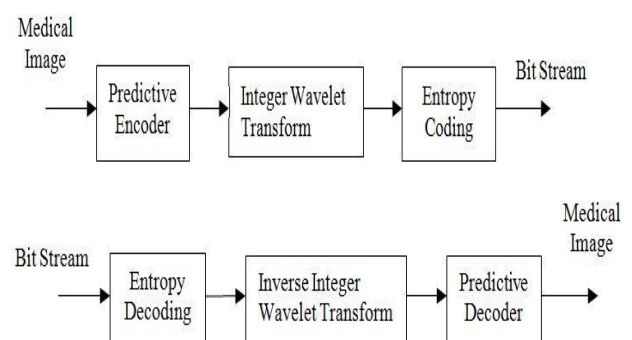
Fig. 1. Block diagram of Encoder and Decoder
