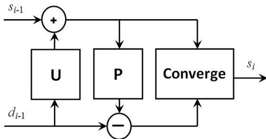
Fig.4. Reverse Lifting Scheme
