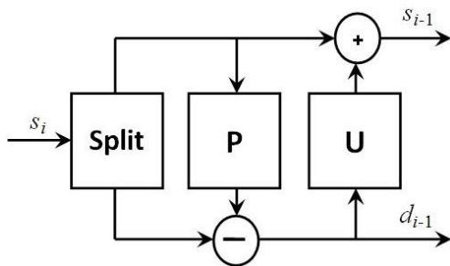
Fig.3. Forward Lifting Scheme
