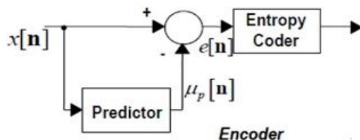
Fig 2. Lossless Predictive Encoder and Decoder
